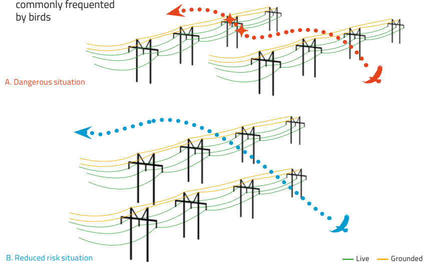
Figure 71. Route planning to avoid risky situations is essential to cut the collision risk to a minimum. Top: The route must consider flight paths and the local topography to avoid risky situations. Bottom: It is practical to combine the routes of neighbouring power lines to create a single obstacle and make it more visible; the efficiency is higher if the towers of the different lines are arranged alternately. Source: adapted from APLIC, 2012 and Pallet et al., 2022
